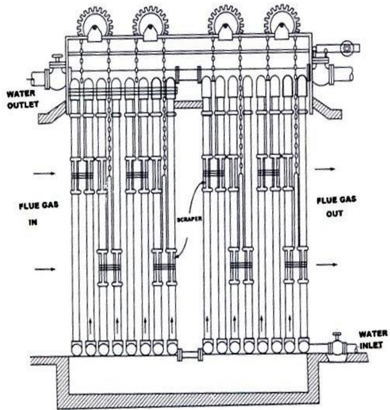
Figure- Economiser
