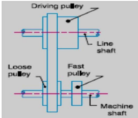
Loose and fast pulleys
