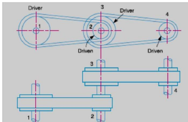
Intermediate pulleys
