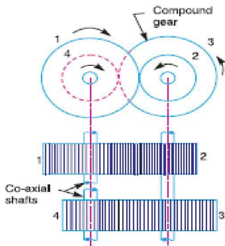
REVERTED GEAR TRAIN DIAGRAM
