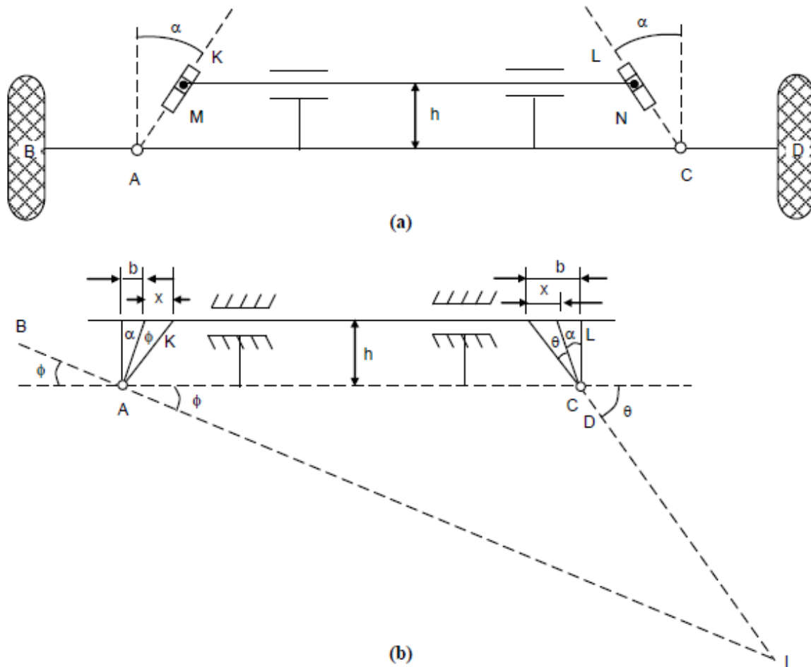
Davis Steering Mechanism
