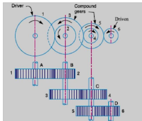
COMPOUND GEAR TRAIN
