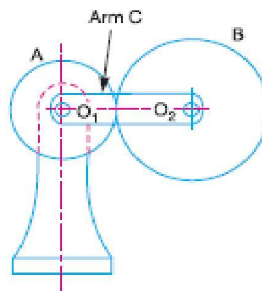
PLANETARY OR EPICYCLIC GEAR TRAIN
