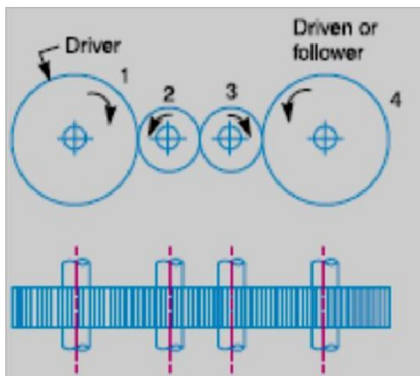
SIMPLE GEAR TRAIN DIAGRAM DIAGRAM
