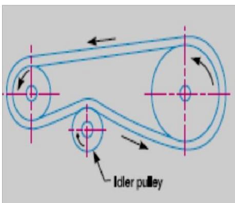
Idler pulleys.
