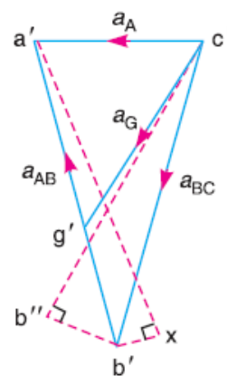
(c) Acceleration diagram.
