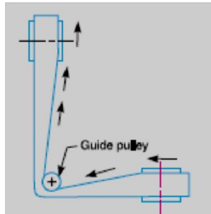
Guide pulleys
